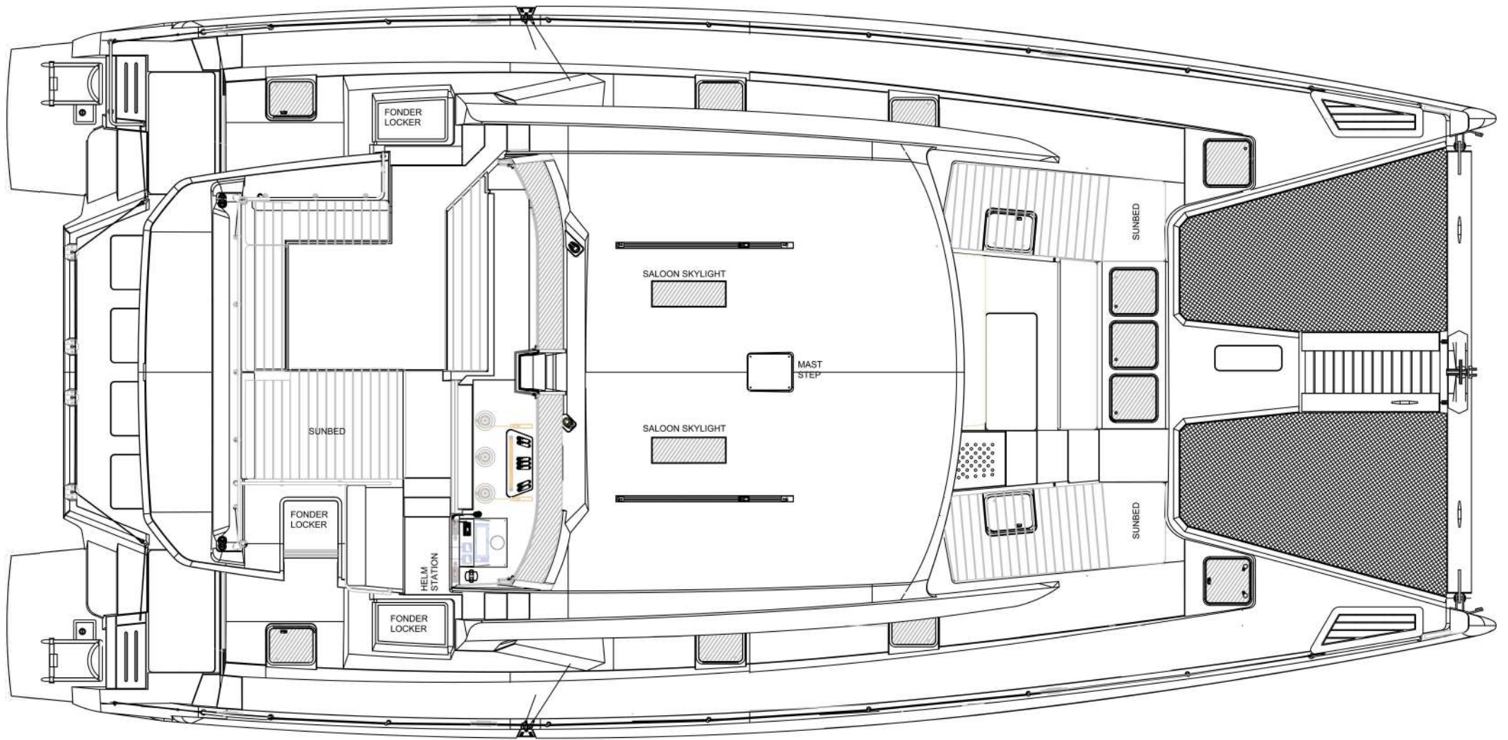
FLYBRIDGE SECTION
