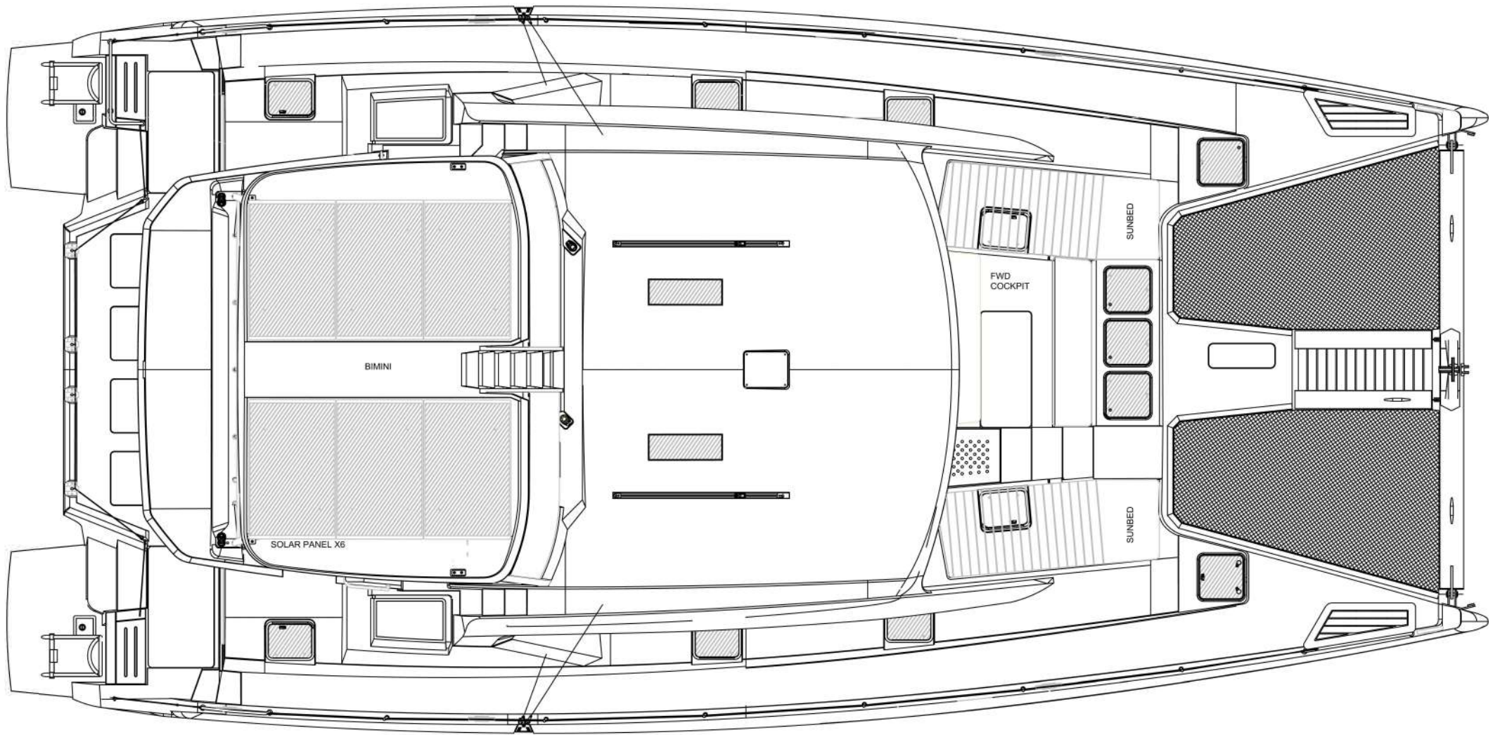
PLAN VIEW
